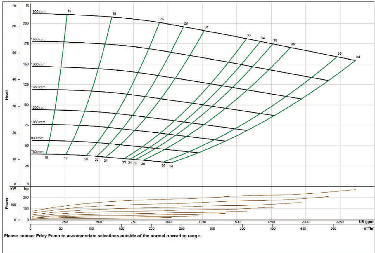
EDDY Pump - 5 Inch HD 5000 Heavy Duty Slurry Pump - Pump Curve
